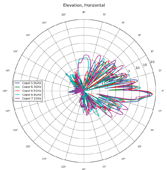
Channel 3 Horizontal Polarization Elevation
